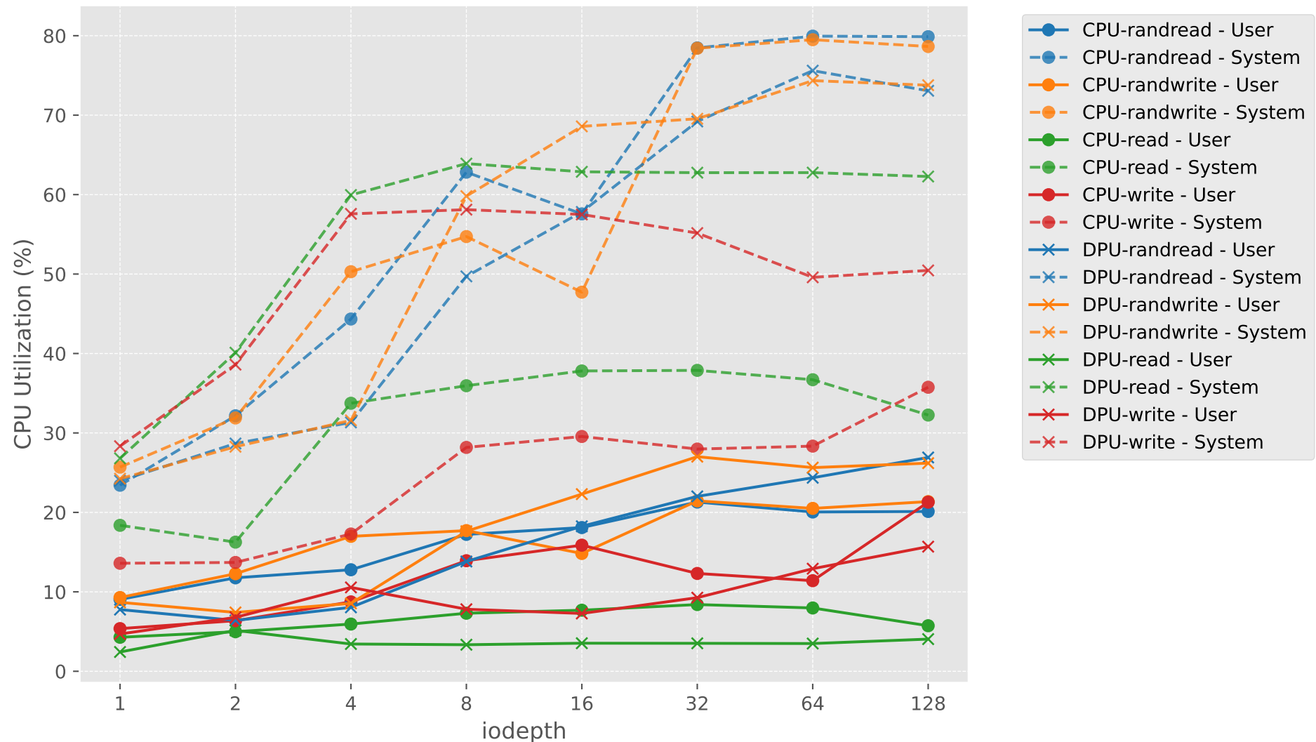
CPU Utilization vs iodepth
